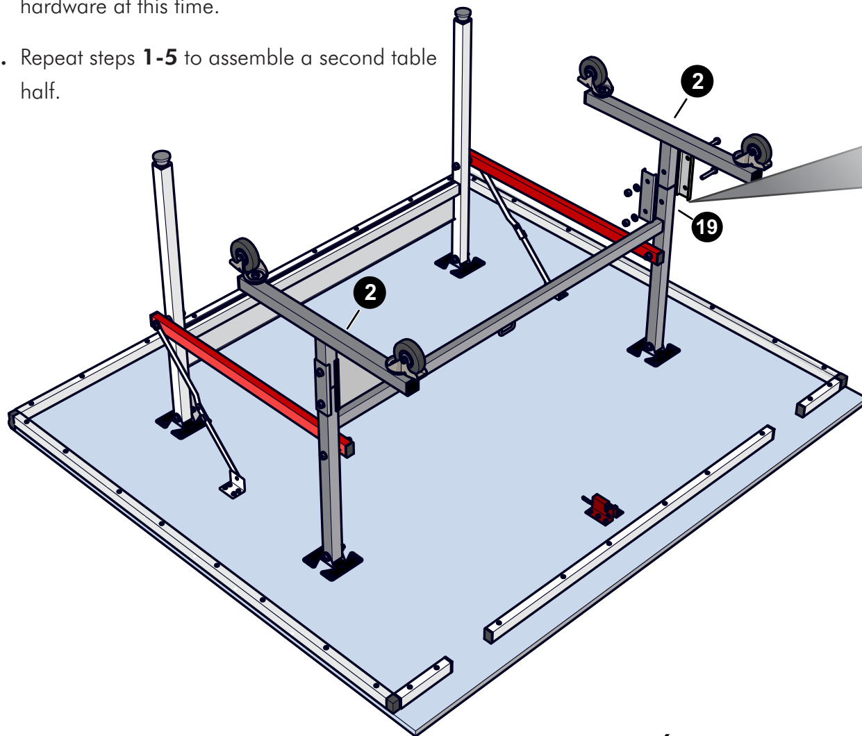
HEX HEAD BOLT 5/16-18 X 1-3/4" 1B-4170-00 (QTY. 8)
