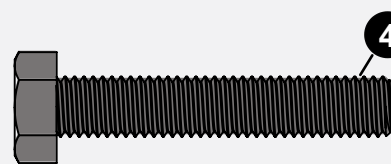
HEX HEAD BOLT 5/16-18 X 1-3/4" 1B-4170-00 (QTY. 8)
