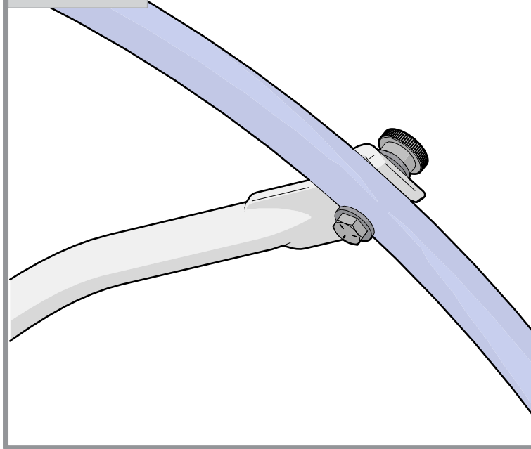
DETAIL B
