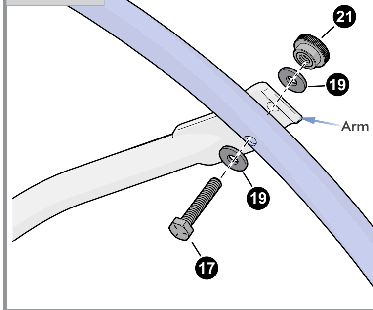
DETAIL A
