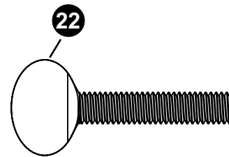
M6 X 1mm X 30mm THUMB SCREW 1B-7242-00 QTY. 2
