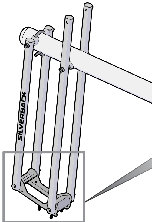
DETAIL A
