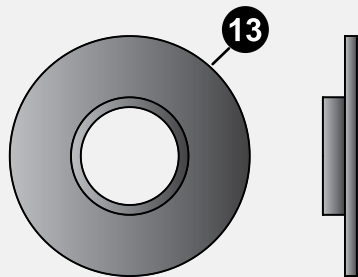
NYLON WASHER WITH ADHESIVE (1/2" ID) 7B-6549-00 (QTY. 4)
