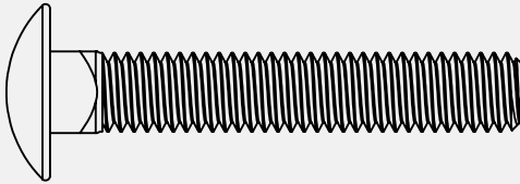
3/8-16 X 2 1/4" CARRIAGE BOLT 1B-7286-00 (QTY. 2)
