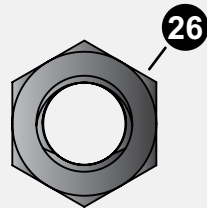
1/2-13 NYLOCK LOCKNUT 2B-6095-10 (QTY. 4)
