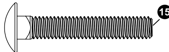
3/8-16 X 2 1/4" CARRIAGE BOLT 1B-7286-00 (QTY. 4)
