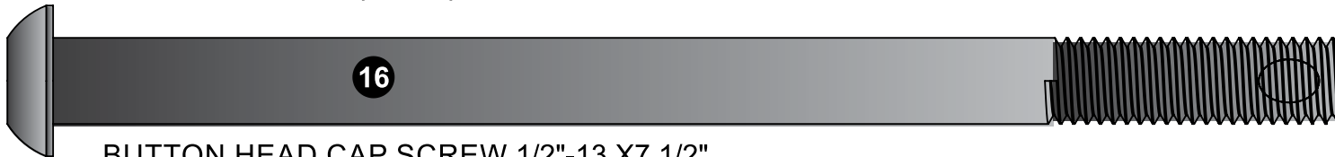
BUTTON HEAD CAP SCREW 1/2"-13 X 7 1/2"
