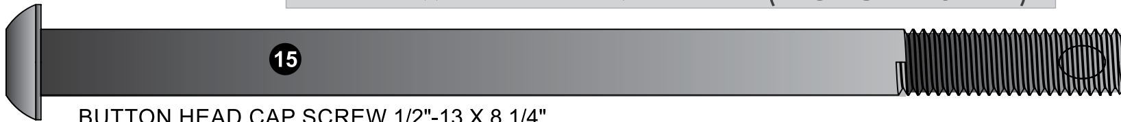
BUTTON HEAD CAP SCREW 1/2"-13 X 8 1/4"
